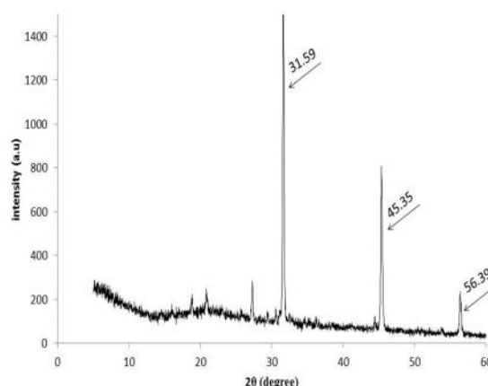
Fig 4: Profile of powder x-ray diffraction of freeze dried AMSC-MP
